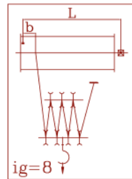
Figure 6: Pulling of cables in angle
