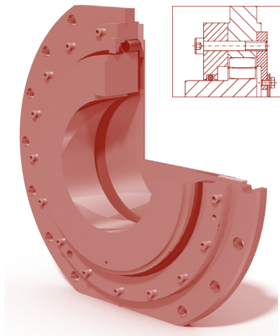
Special flange without carrier faces
