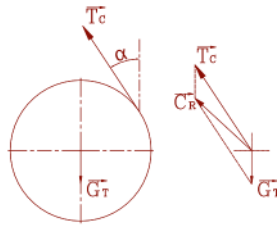
Figure 6: Pulling of cables in angle
