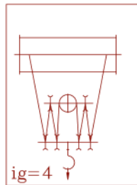
Figure 7: Examples of hoist ratios
