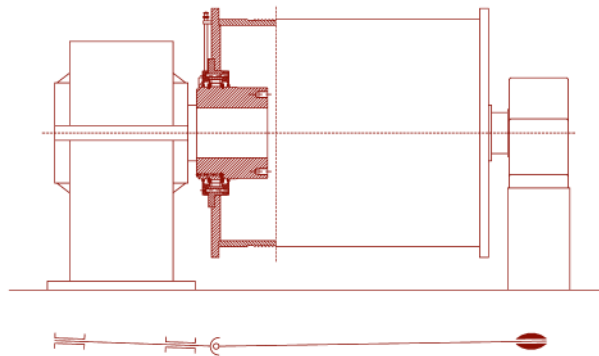
Figure 2: articulated joint Reducer-Drum
